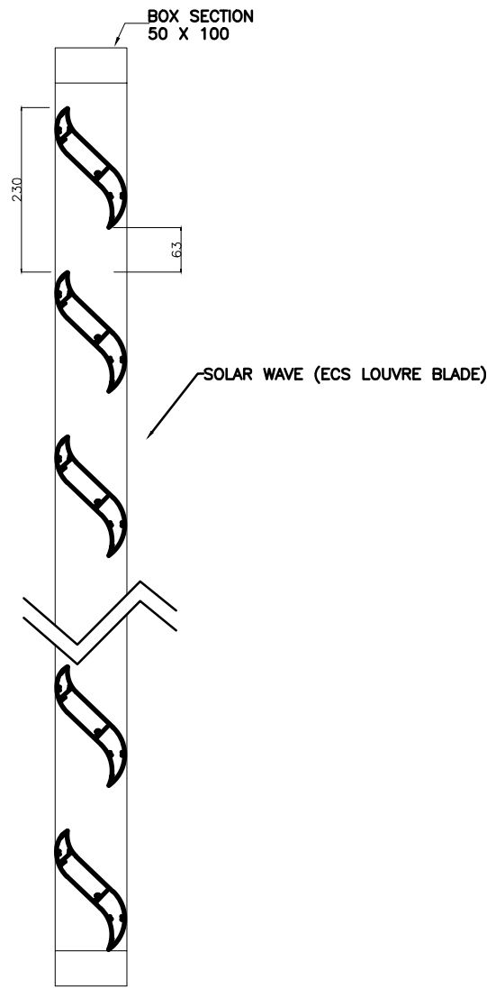
SOLAR SHADE VERTICAL VIEW BOX ENCLOSURE
