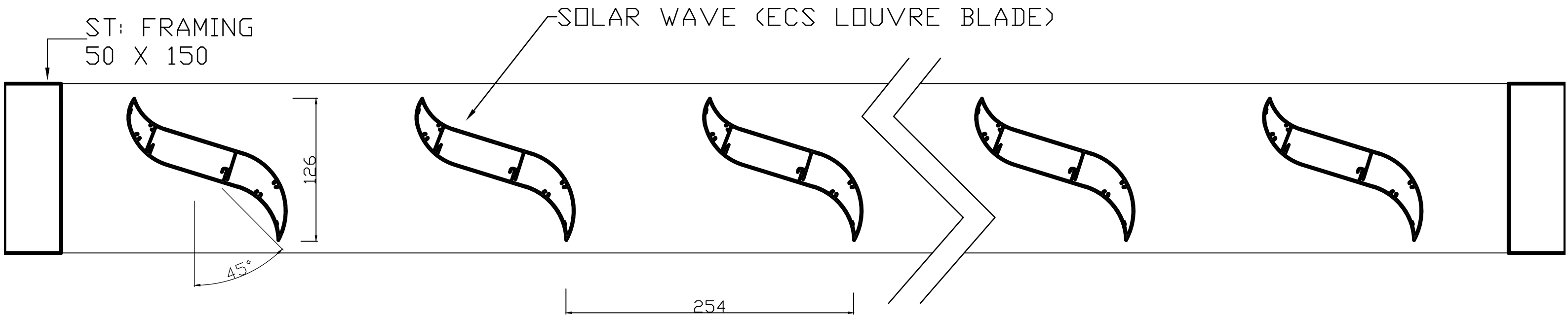
TYPICAL SECTION THROUGH SOLAR SHADE HORIZONTAL VIEW
