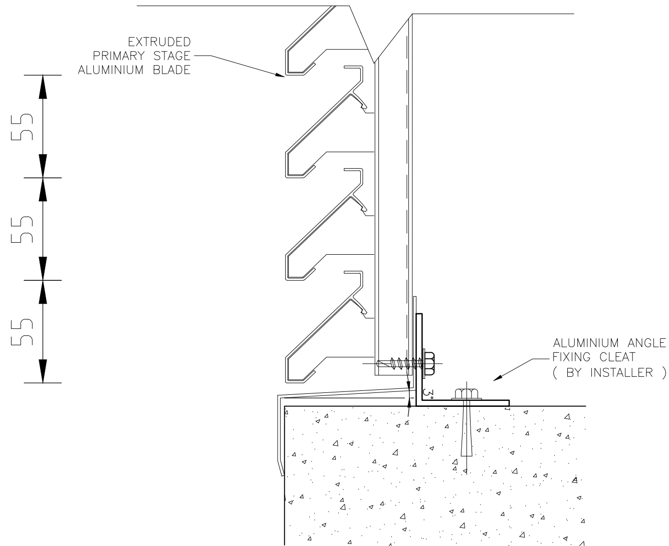
ELEMENT CONTROL SYSTEMS 55 PRIMARY STAGE LOUVRE SILL INTO MASONRY
