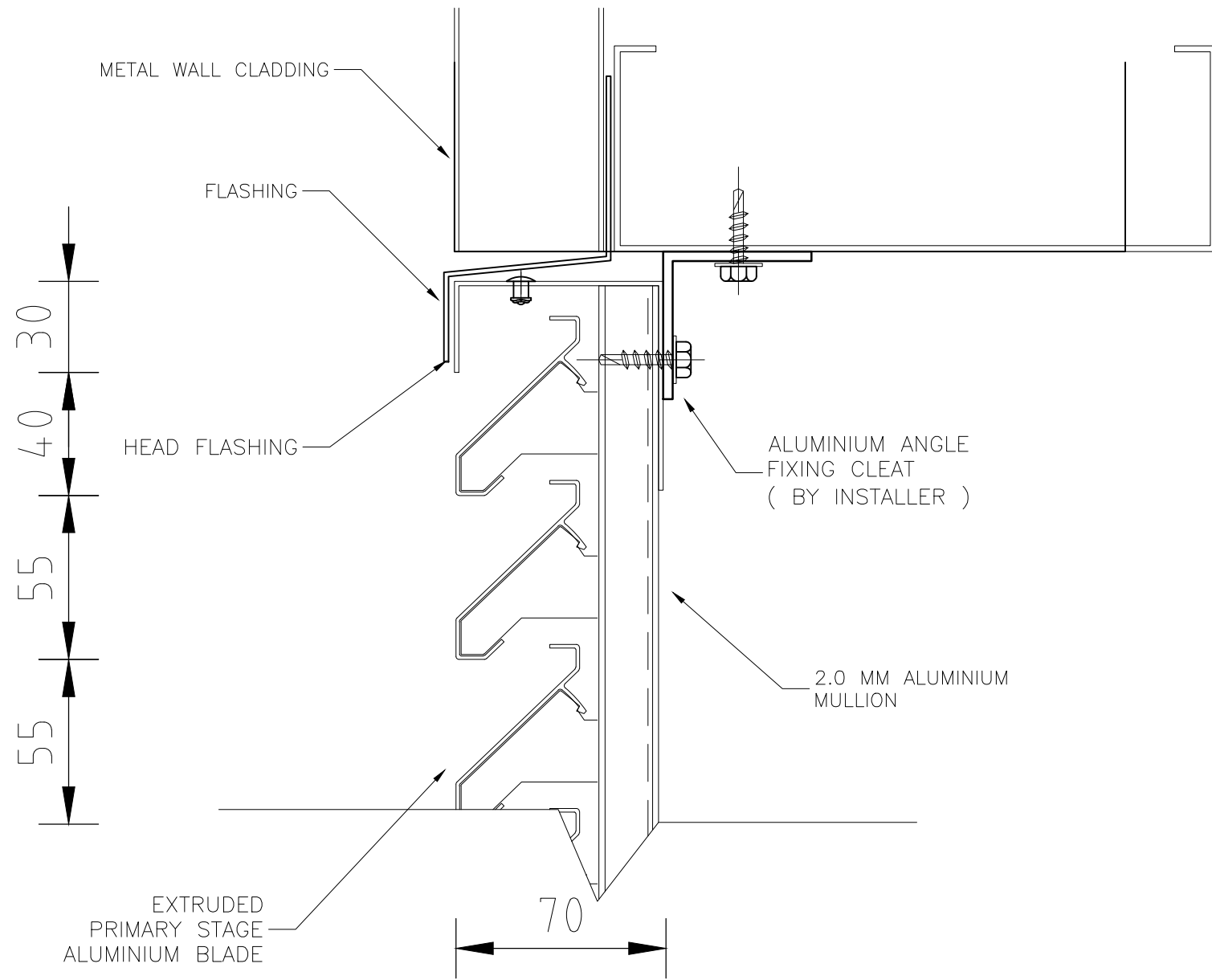
ELEMENT CONTROL SYSTEMS 55 PRIMARY STAGE LOUVRE HEAD INTO CLADDING
