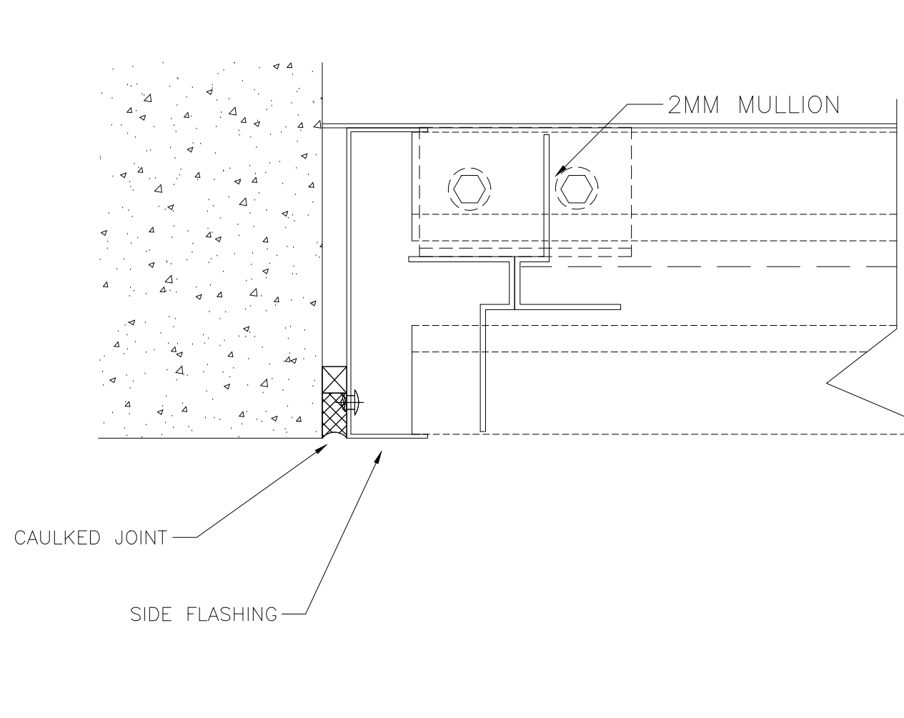
JAMB DETAIL BIRDMESH OR BLANKING PANEL INTO MASONRY
