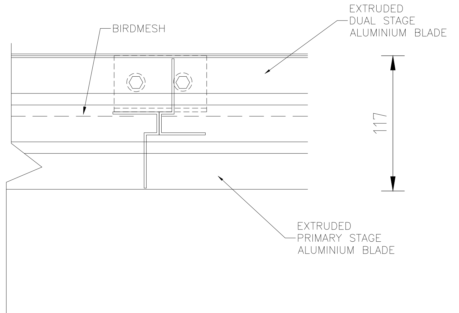
INTER MULL DETAIL BIRDMESH OR BLANKING PANEL INTO MASONRY
