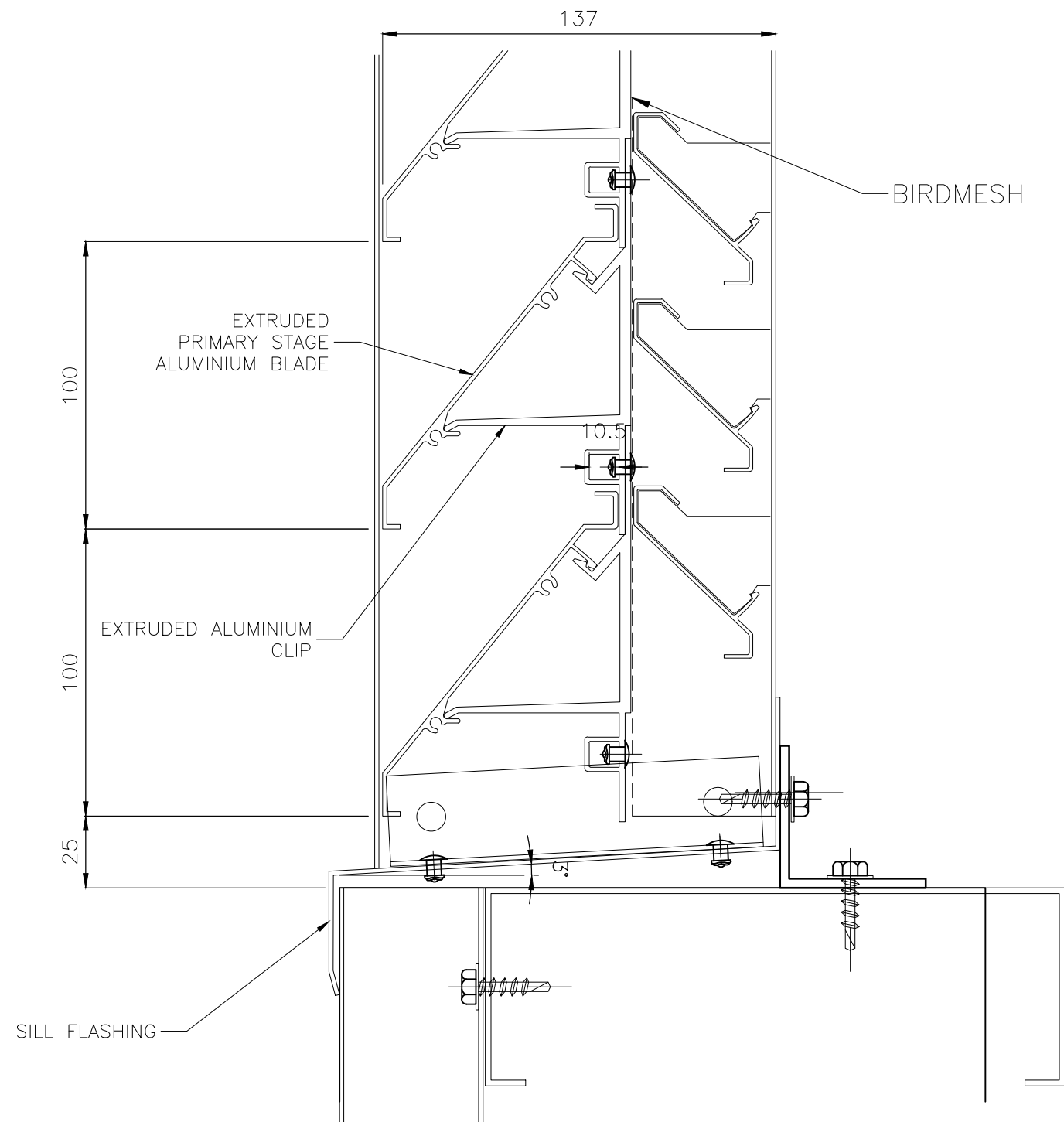
ELEMENT CONTROL SYSTEMS 100 DUAL STAGE LOUVRE SILL SILL INTO CLADDING
