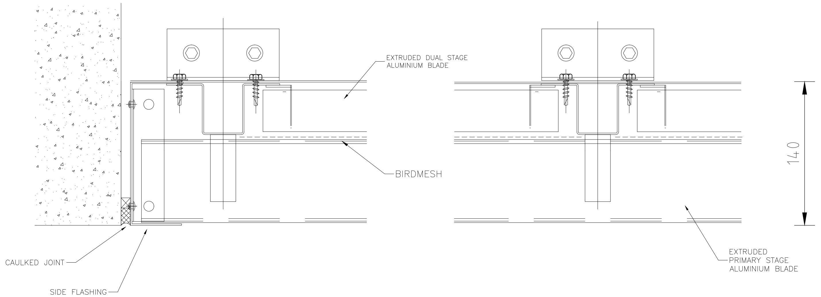
JAMB DETAIL BIRDMESH OR BLANKING PANEL INTO MASONRY
