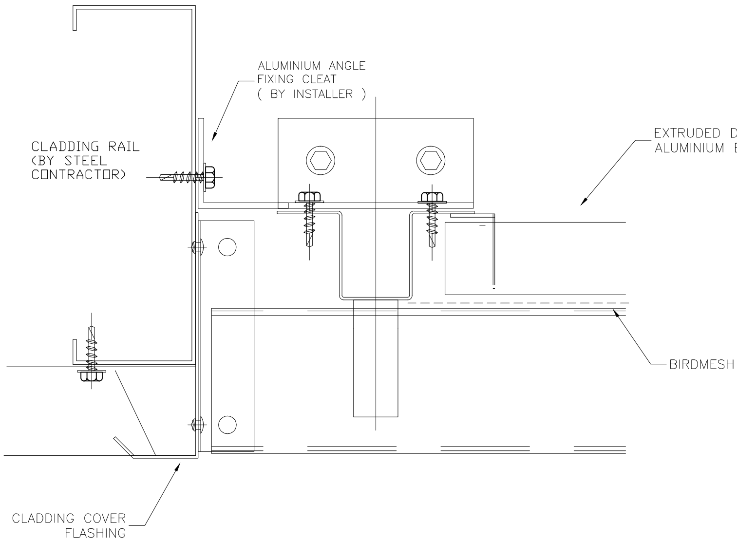
JAMB DETAIL BIRDMESH
