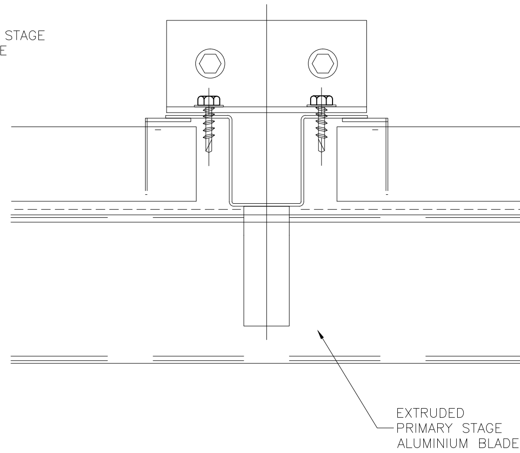
INTER MULL DETAIL BIRDMESH
